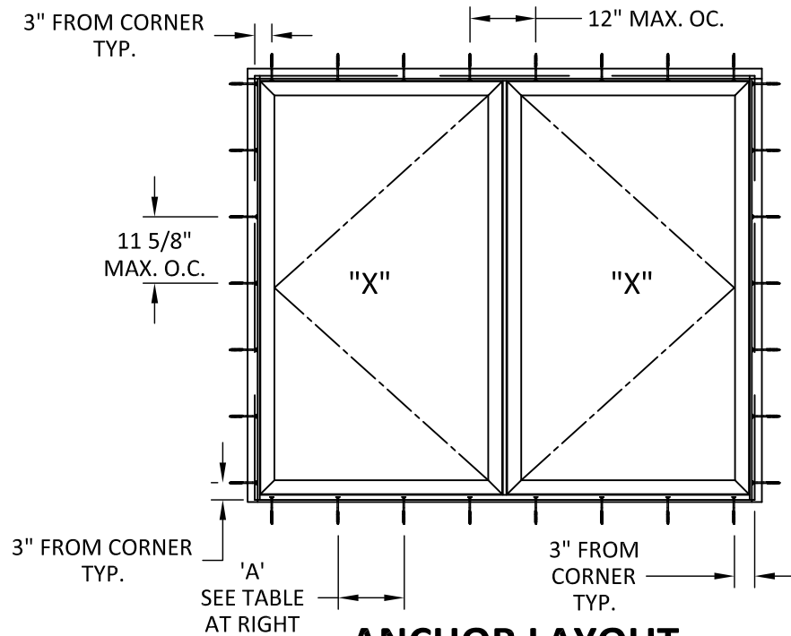
ANCHOR LAYOUT FRENCH CASEMENT ALL INSTALLATIONS
