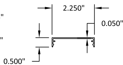
20 COVER 6063-T5
