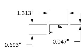
12 FIXED SNAP COVER 6063-T5
