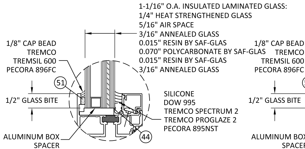
GLAZING DETAIL A1
