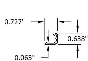
13 VENT GLASS STOP 6063-T5
