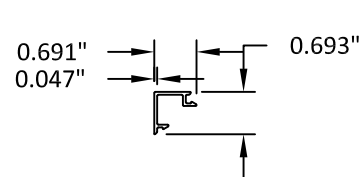
14 VENT SNAP COVER 6063-T5
