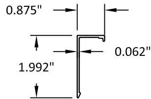
64 ANCHOR CLIP COVER 6063-T5
