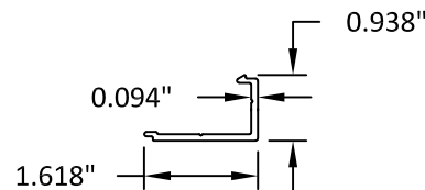
68 1" X 1 11/16" CLIP 6063-T5 CONTINUOUS
