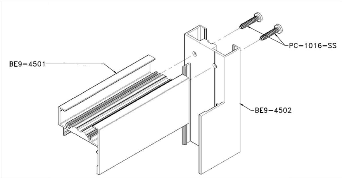
FRAME CORNER CONSTRUCTION TYPICAL
