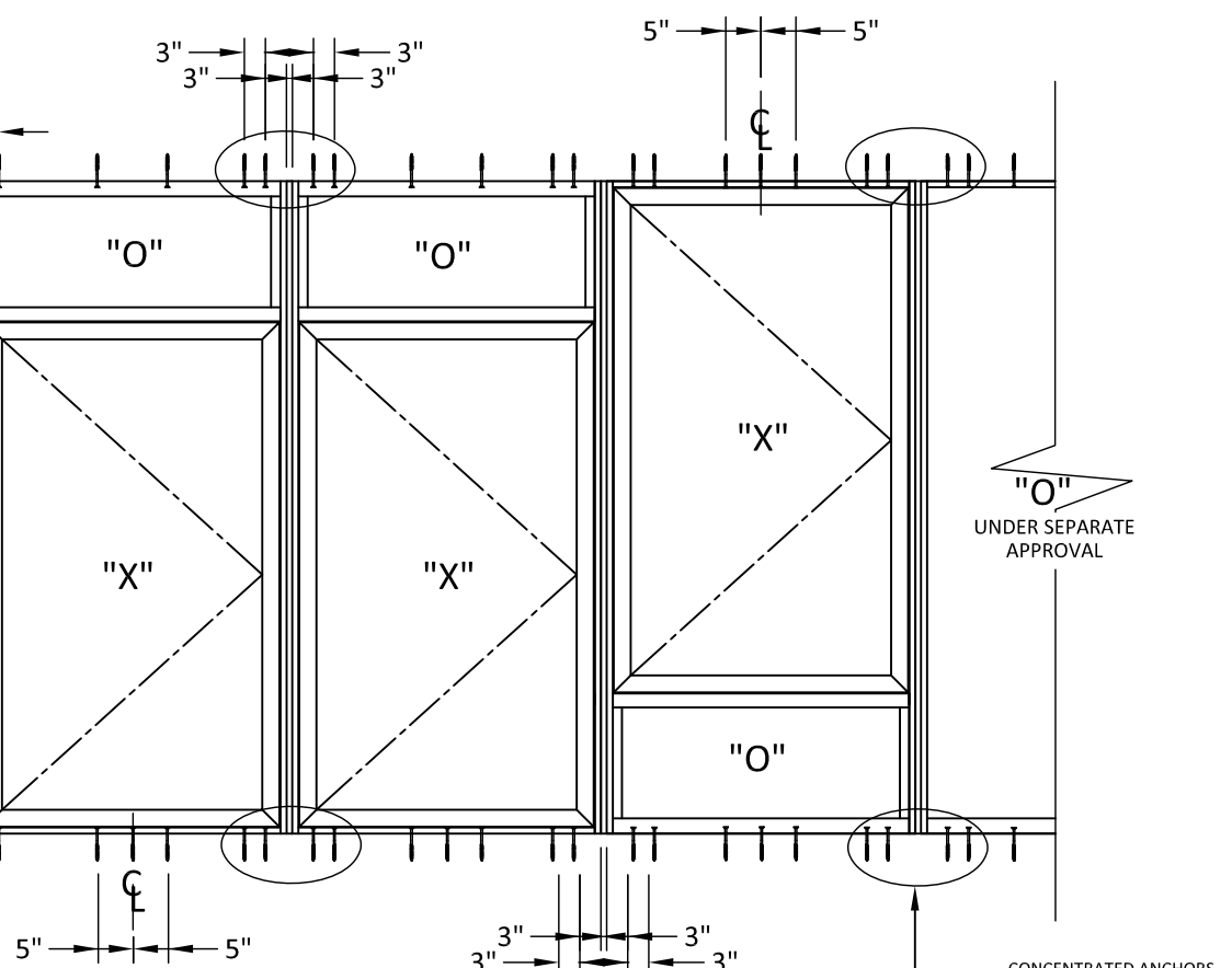
ANCHOR LAYOUT RECEPTOR INSTALLATIONS
