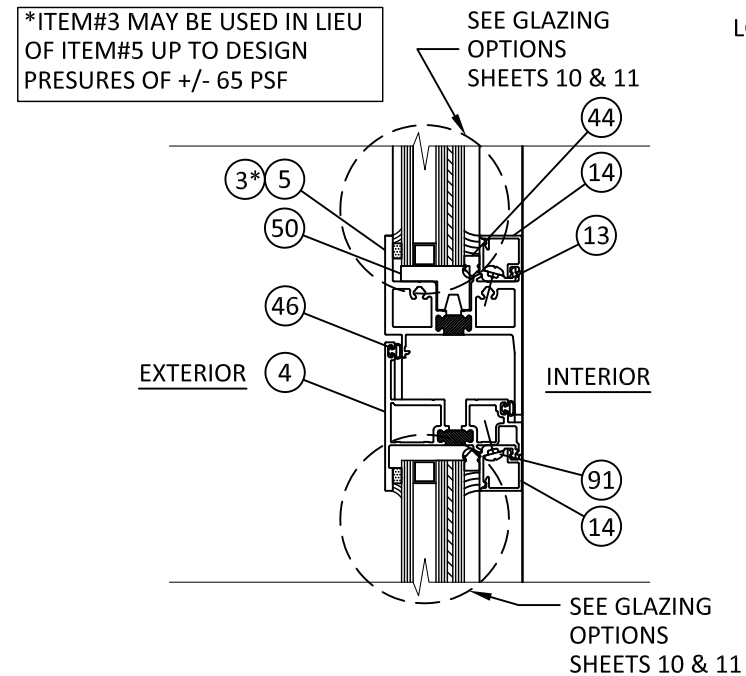
V9 VERTICAL SECTION INTEGRAL MULLION-TYP. FIXED OVER CASEMENT
