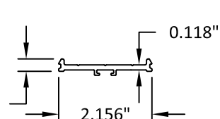
9 PRESSURE BAR 6063-T5
