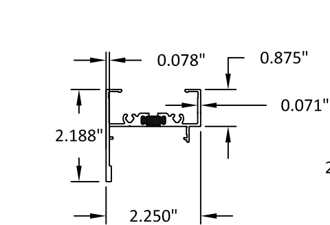
1 FRAME HEAD & SILL 6063-T5
