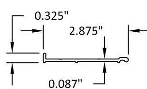
16 SILL TRIM BASE 6063-T5
