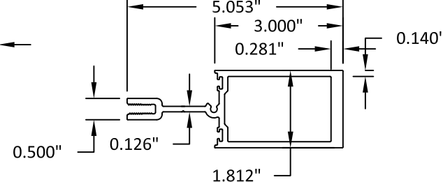
17 STACKING MULLION 6063-T5
