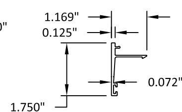
18 RECEPTOR STOP 6063-T5
