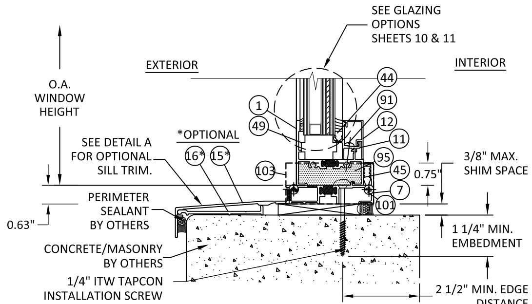
A 4 VERTICAL SECTION FIXED SILL - CONCRETE/MASONRY RECEPTOR & SILL FLASHING - TYP.
