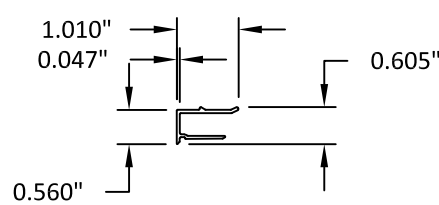
22 FIXED GLASS SNAP COVER 6063-T5
