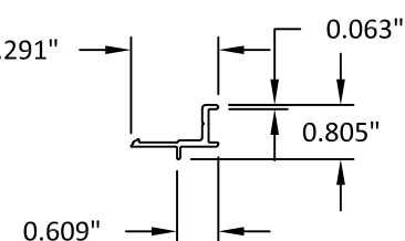
21 FIXED GLASS STOP 6063-T5
