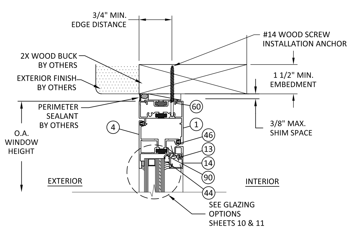
O7 VERTICAL SECTION VENT HEAD - 2X WOOD BUCK THROUGH FRAME - TYP.
