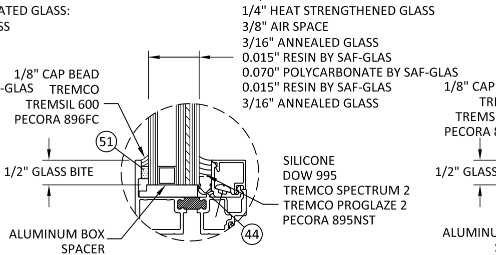
GLAZING DETAIL A2
