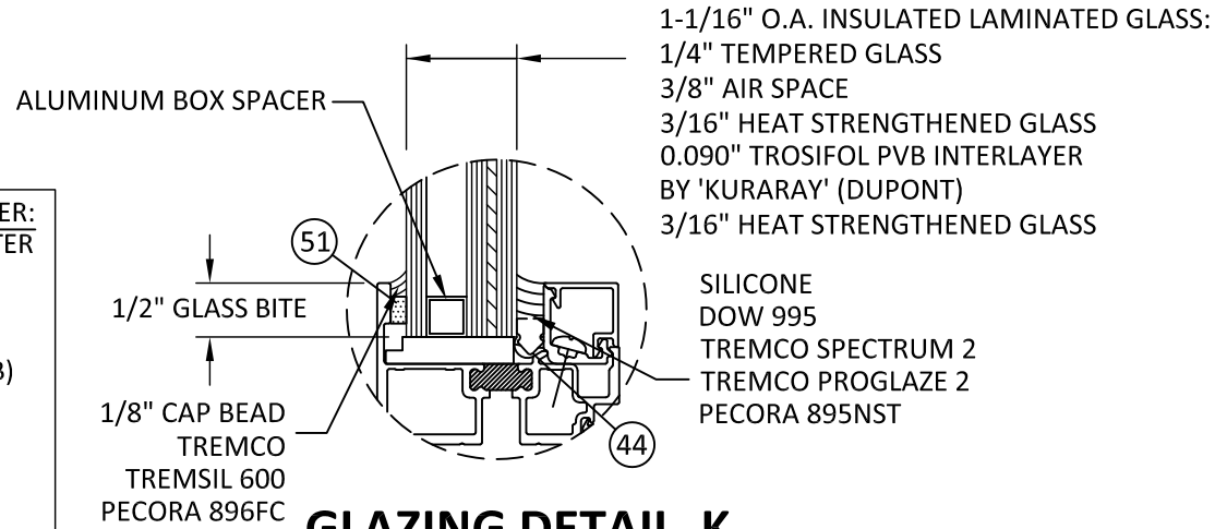
GLAZING DETAIL K
