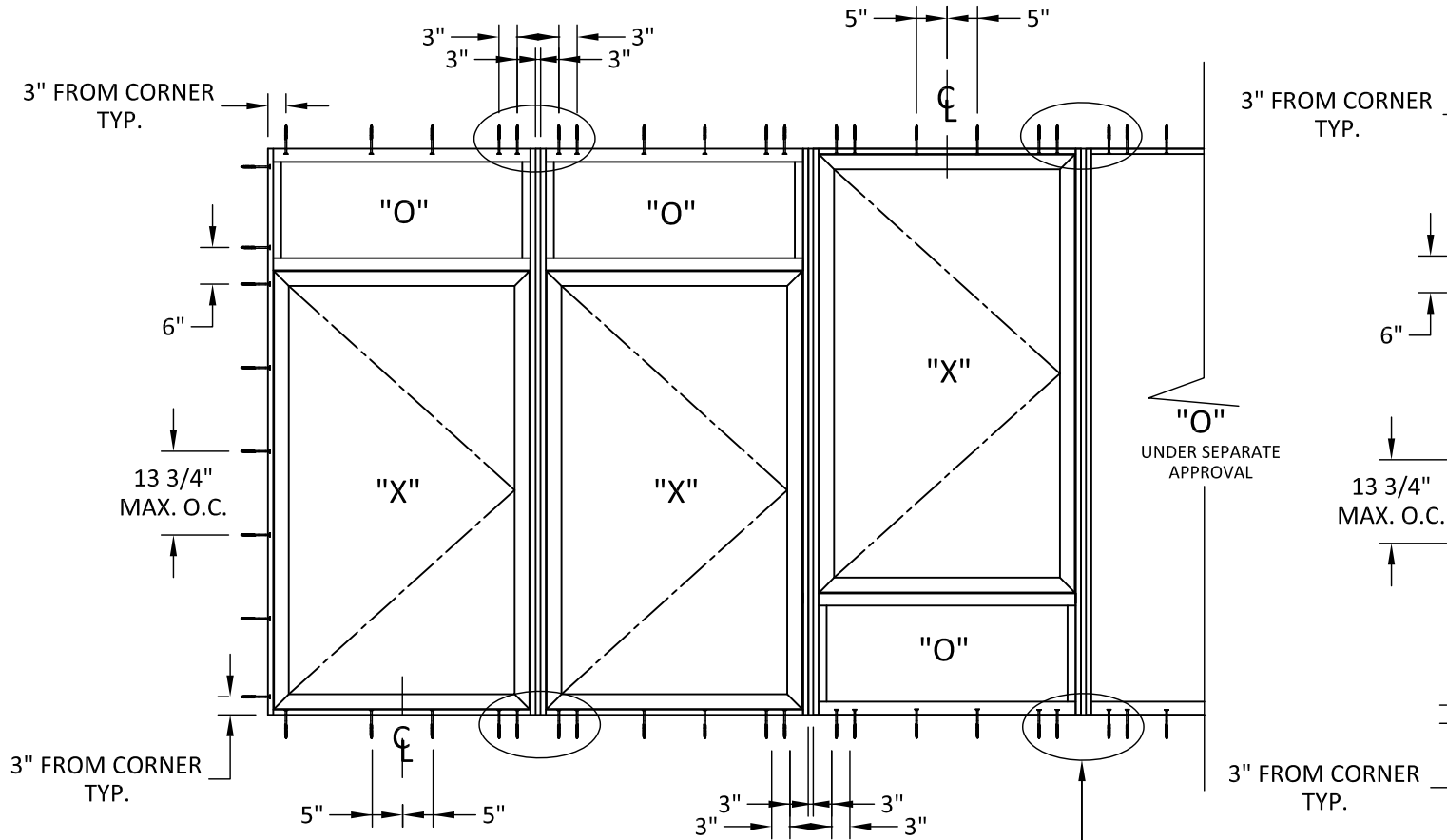
ANCHOR LAYOUT STRAP, CLIP, THRU FRAME, OR TRIM/CLIP INSTALLATIONS
